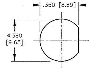
SUGGESTED MOUNTING CONFIGURATION
