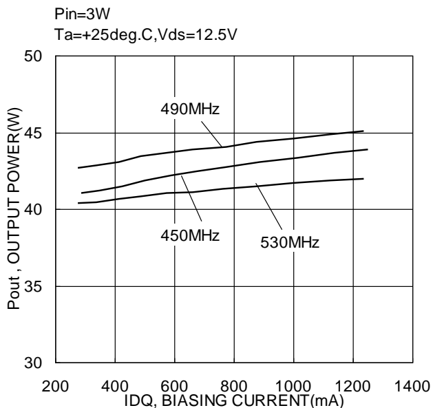
Output Power versus Biasing Current
