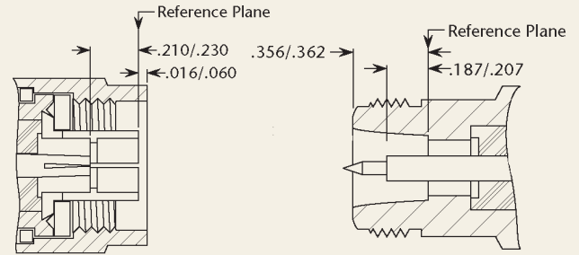
Plug (male)
