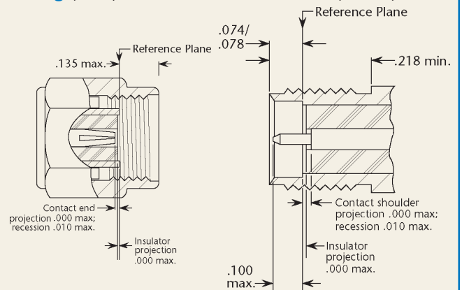
Plug (male)
