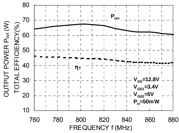
OUTPUT POWER, TOTAL EFFICIENCY, versus FREQUENCY
